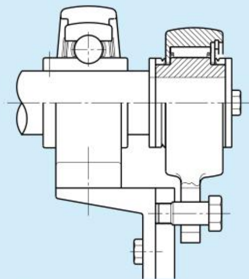
Typical Installation 1
