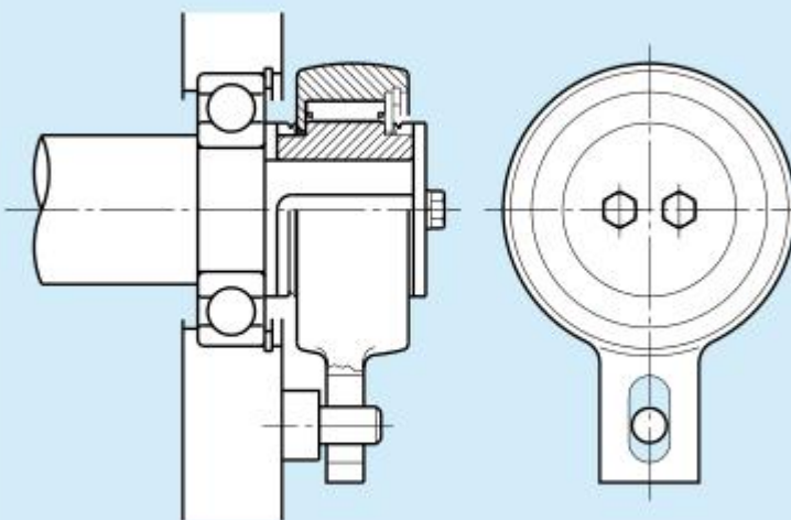
Typical Installation 2
